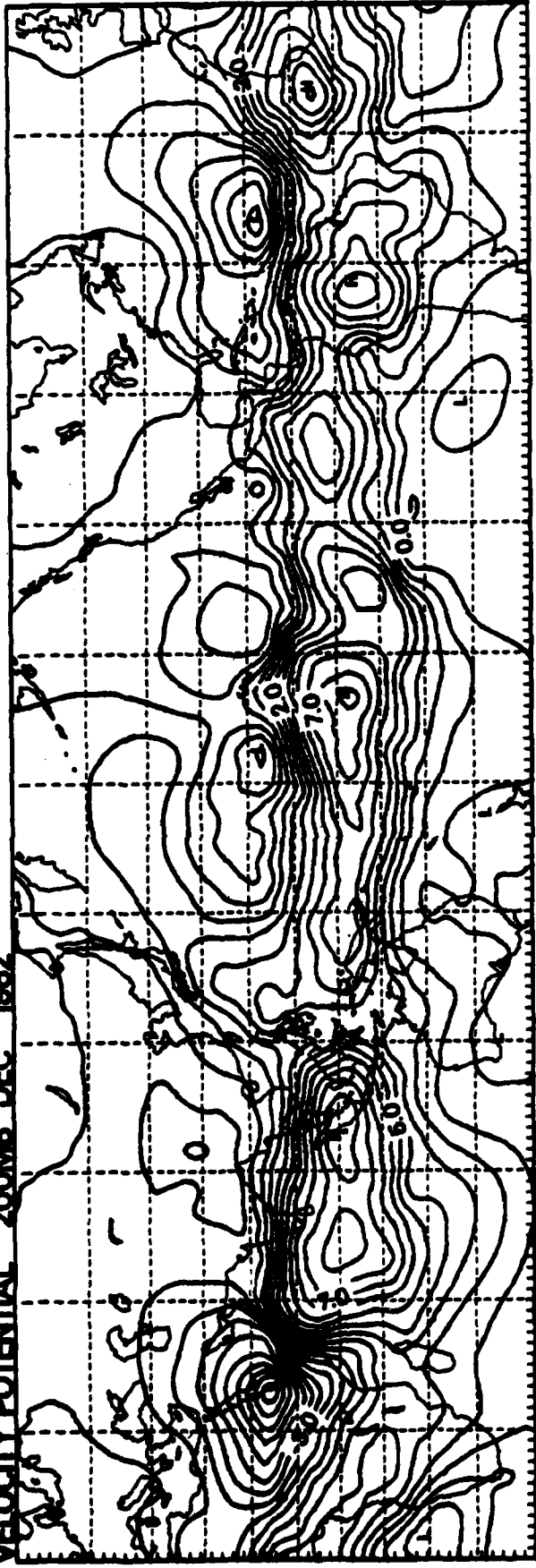
VELOCITY POTENTIAL 200MB DEC 1982
